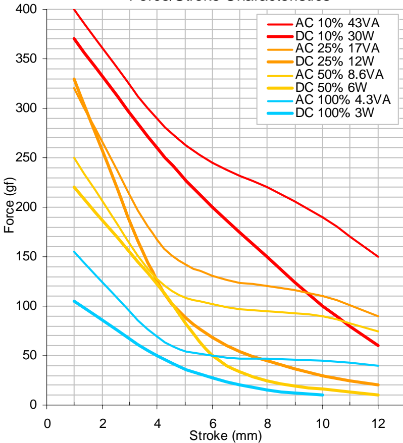
Force/Stroke Characteristics
